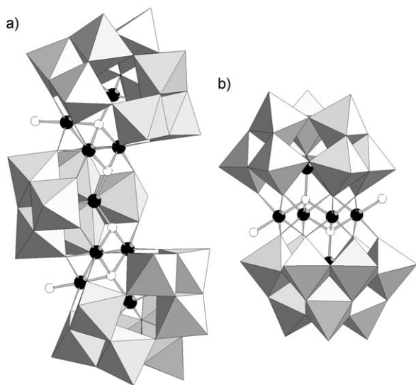
Figure 1. Mixed polyhedral and ball-and-stick representations of a) complex 1 and b) complex 2 . Gray octahedra \text{WO}_6 , black spheres Fe, white spheres O.
